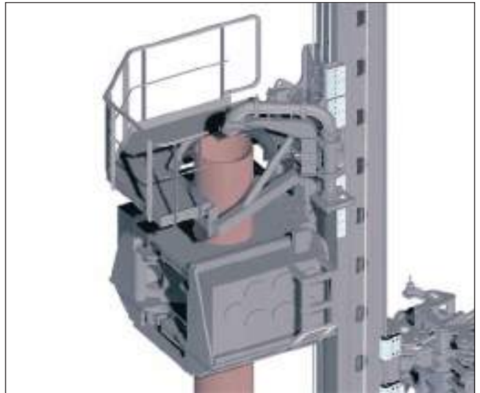
Ring vibrator with platform and concreting system
